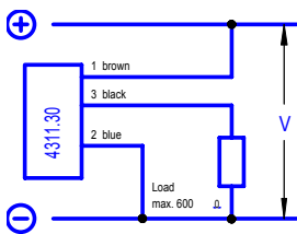
4 - 20 mA current output
